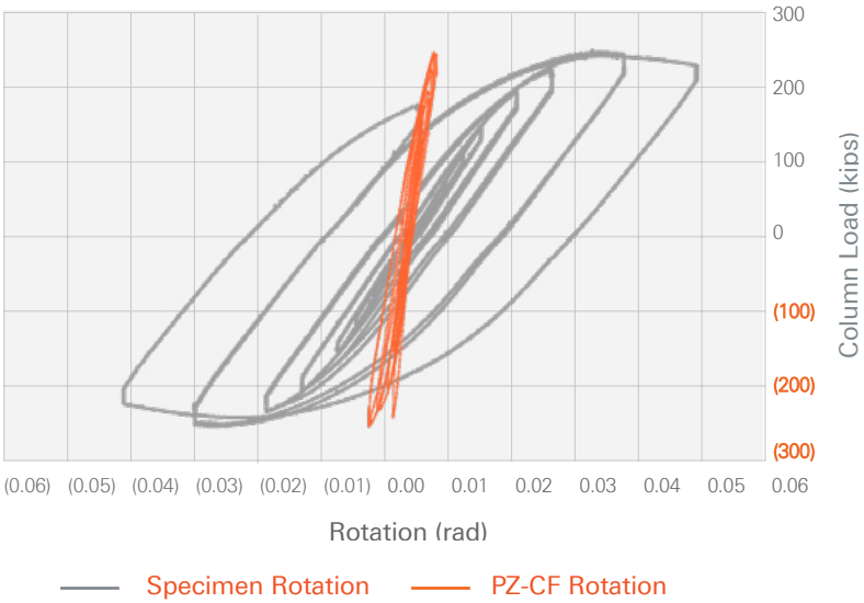
Load vs Rotation W30x108xRBS ConXL Bi-Axial Test #2101A.
